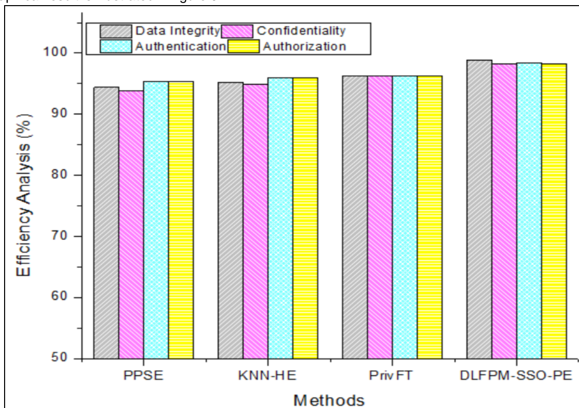
Figure 6 :Efficiency Analysis
