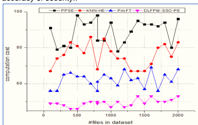
Figure 2: Computation cost
