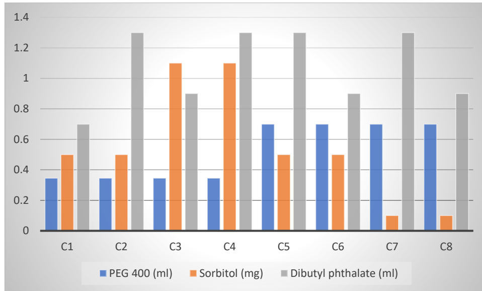
Figure 2: Composition of Coating Formulation
